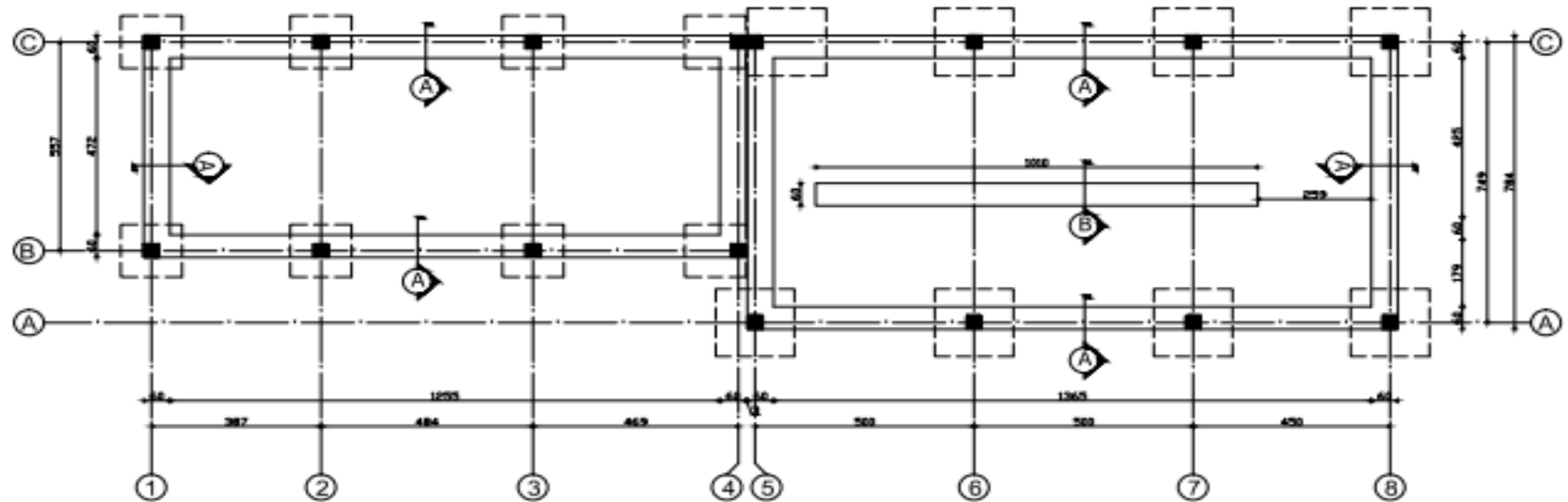
Ring Beam & Stone Found.. Plan:
