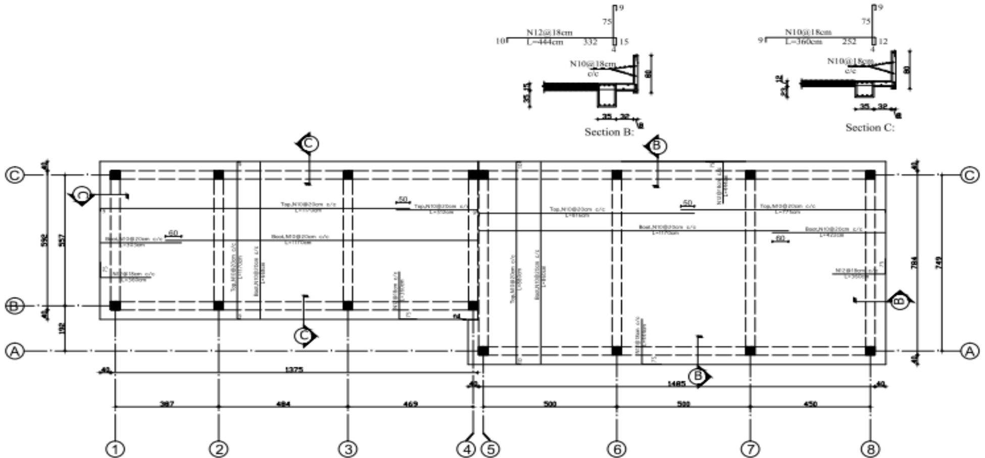
RCC Slab Plan:
