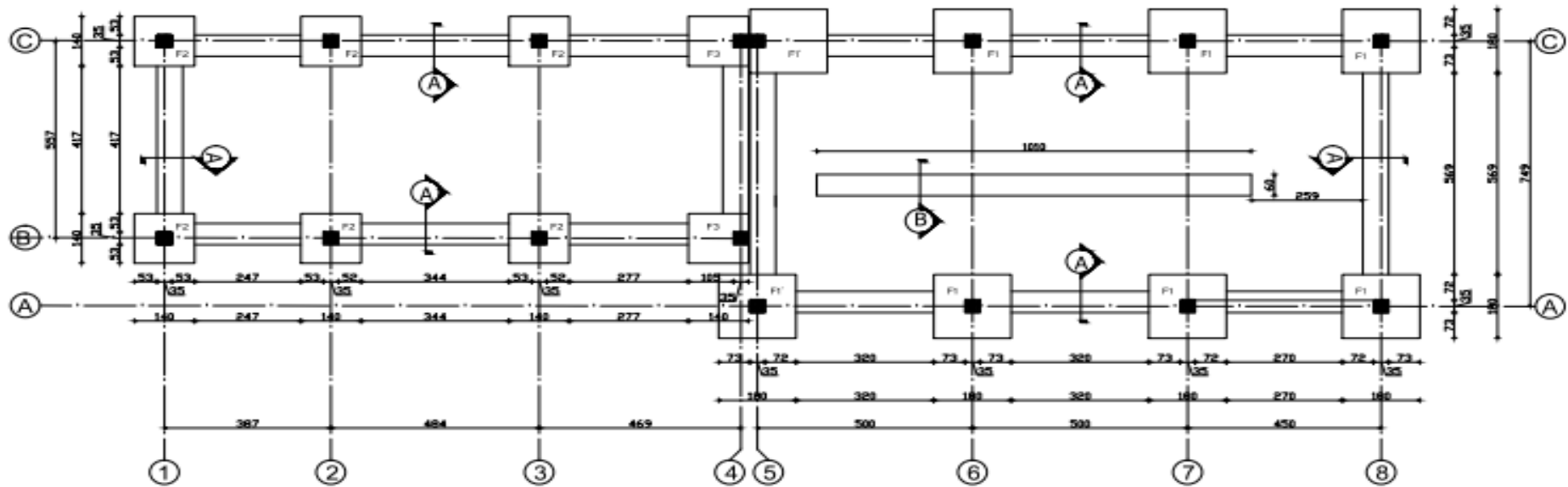
Foundation Plan:
