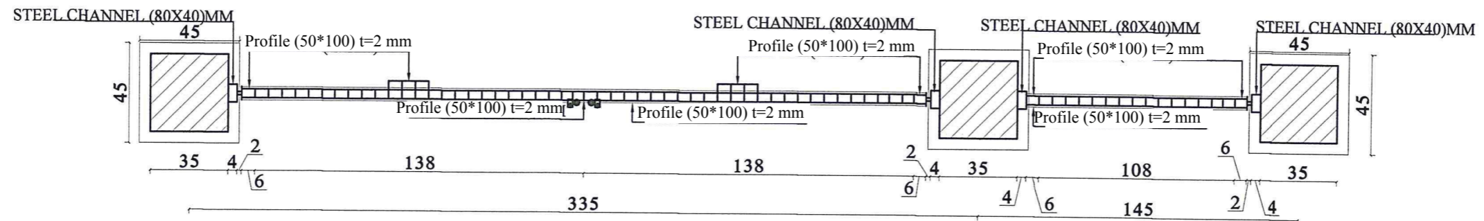
PLAN FOR DOORS
