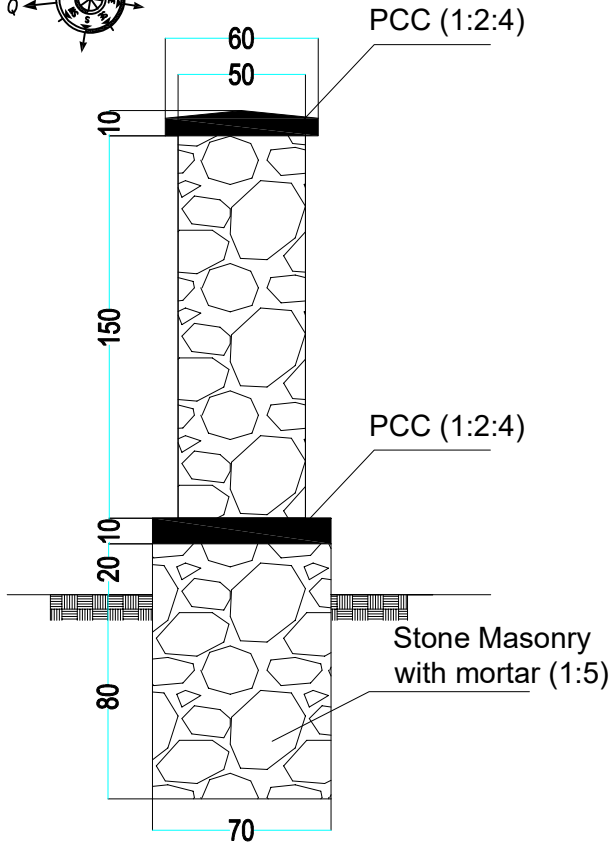
Stone Boundary Wall Section A-A
