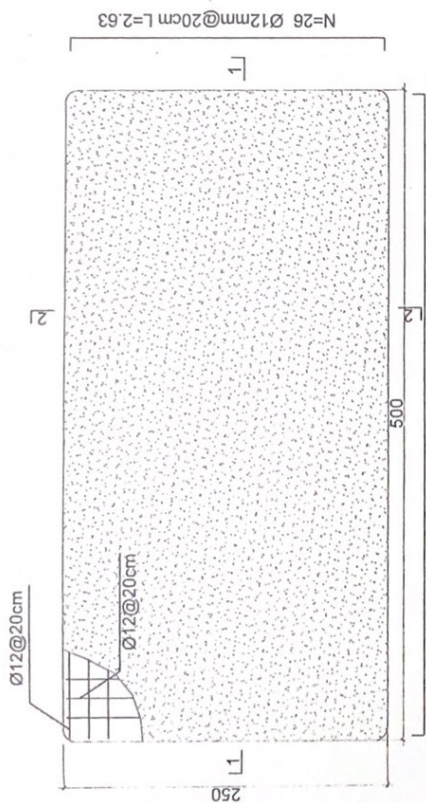
Generator Foundation
