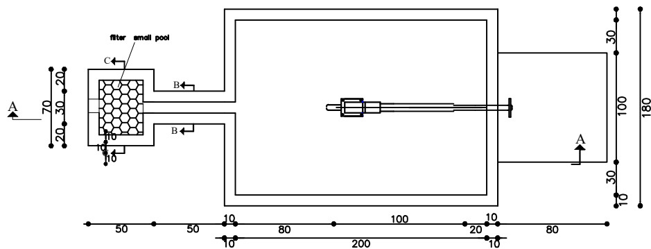
PLAN OF HAND WELL WITH APRON
